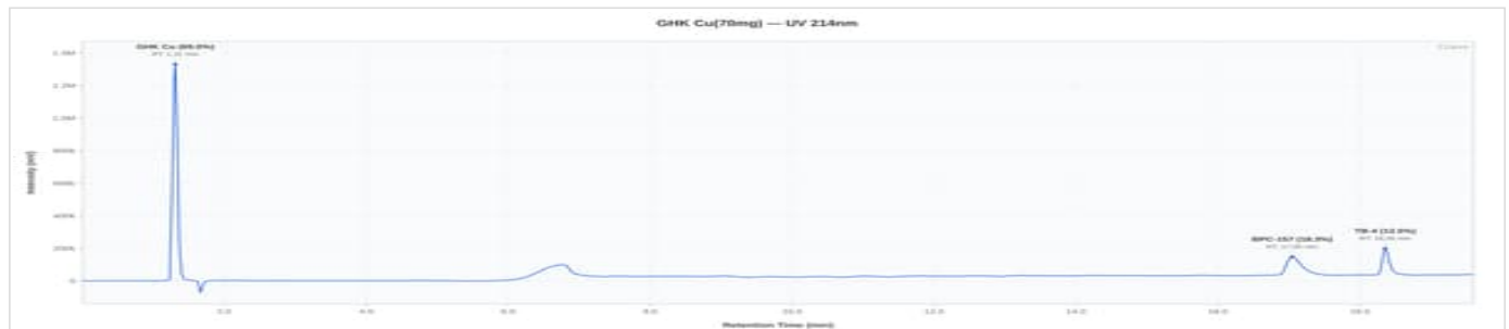
GLOW 70mg - 70GLOW2608BT01: UV Chromatogram
