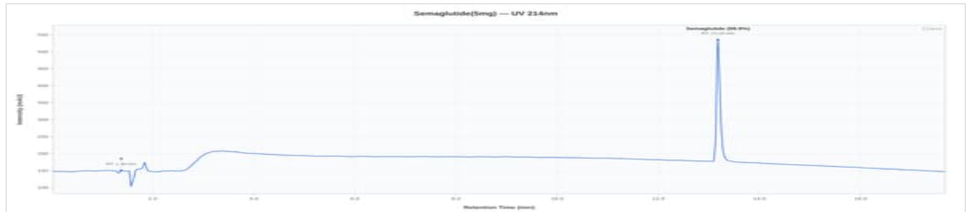
Semaglutide 5mg - 5SEMA2608BT01: UV Chromatogram
