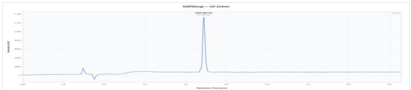
DSIP 5mg - 5DSIP2608BT01: UV Chromatogram
