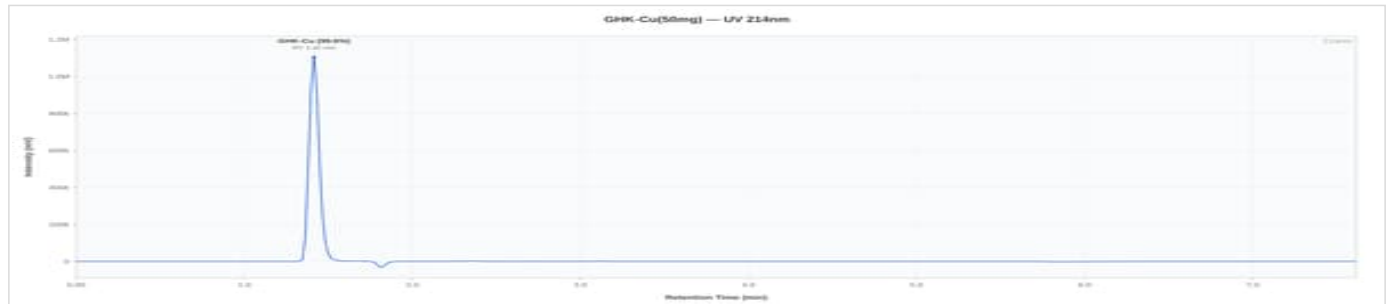
GHK-Cu 50mg - 50GHKC2608BT01: UV Chromatogram
