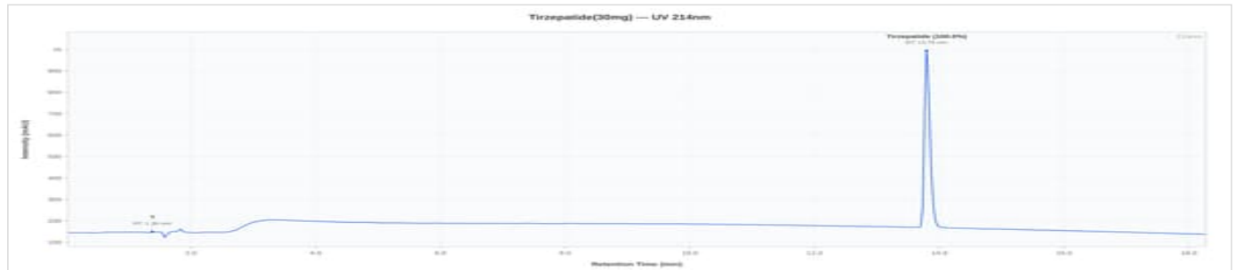
Tirzepatide 30mg - 30TIRZ2608BT01: UV Chromatogram
