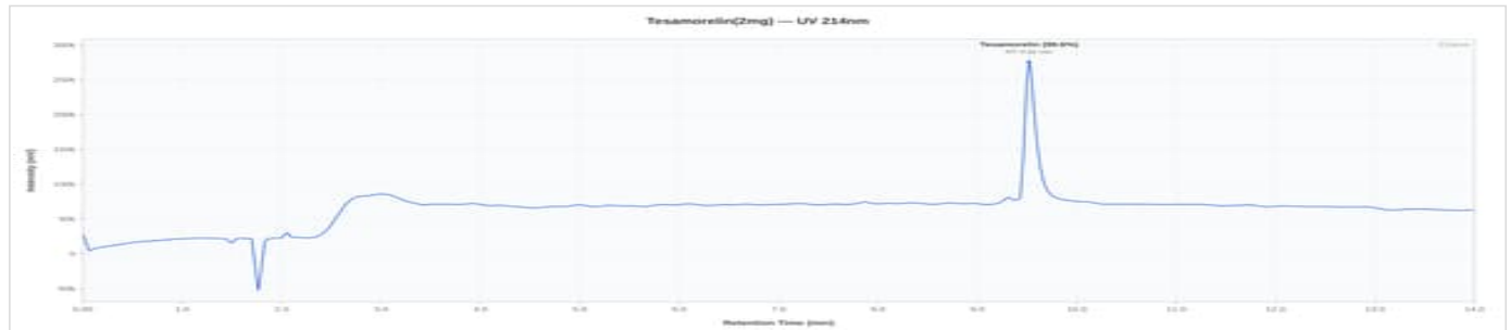
Tesamorelin 2mg - 2TESA2608BT01: UV Chromatogram
