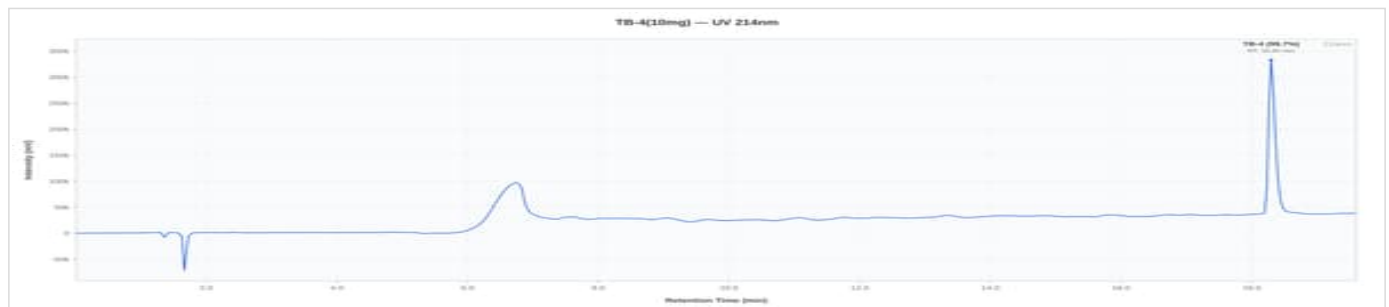
TB-500 10mg - 10TB502608BT01: UV Chromatogram
