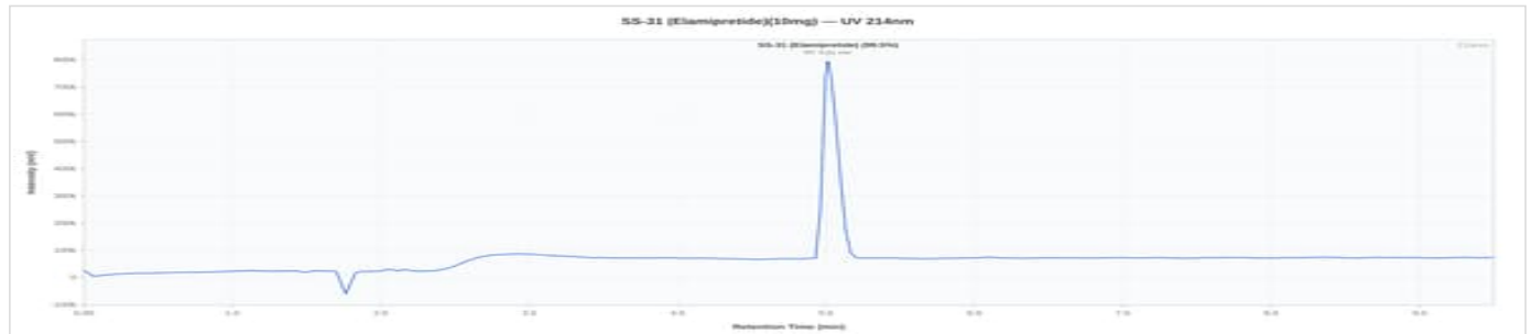
SS-31 10mg - 10SS312608BT01: UV Chromatogram
