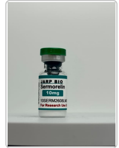
Sermorelin 10mg - 10SERM2608LM01
