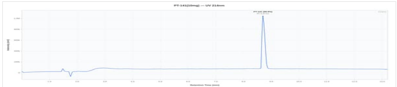
PT-141 10mg - 10PT142608BT01: UV Chromatogram
