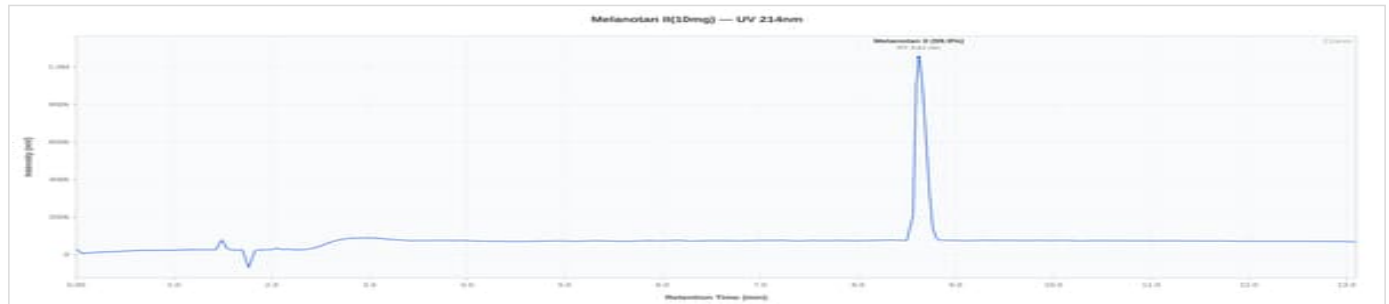
Melanotan 2 10mg - 10MT022608BT01: UV Chromatogram
