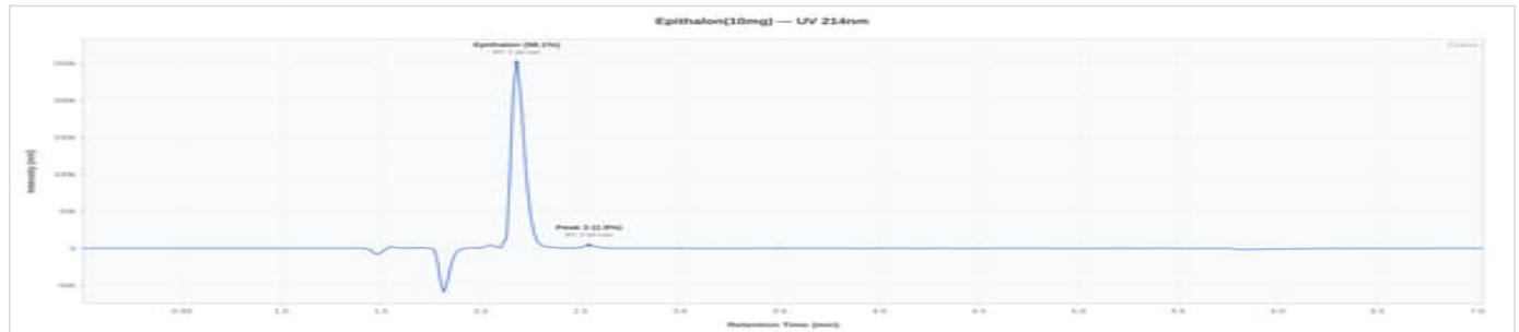
Epithalon 10mg - 10EPIT2608BT01: UV Chromatogram
